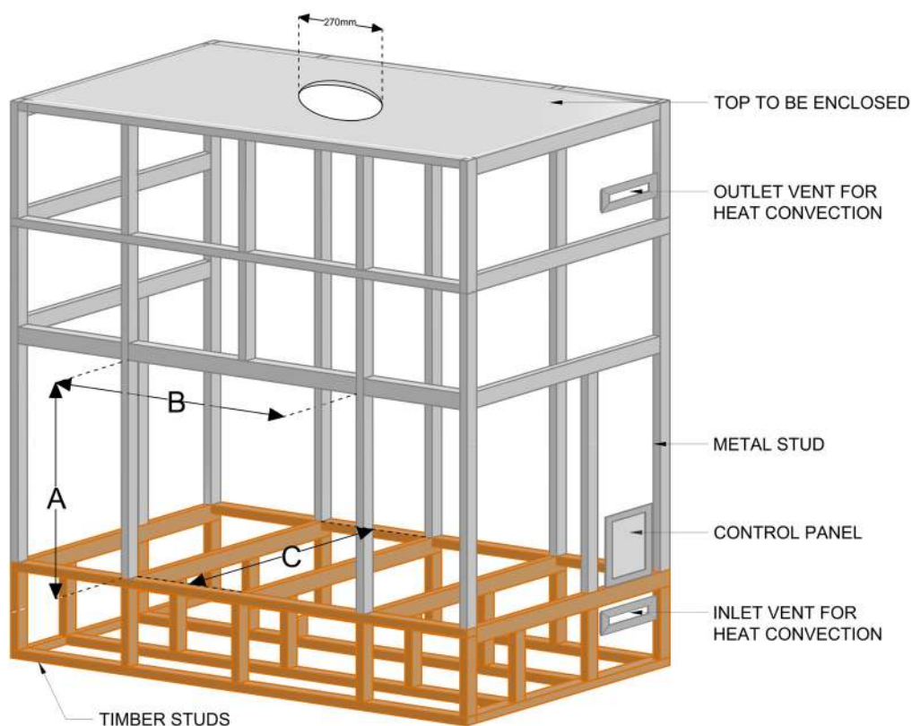
Figure 1.9 (Metal framing)
