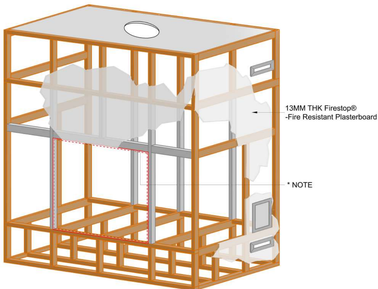
Figure 1.7 (Cladding Material)
