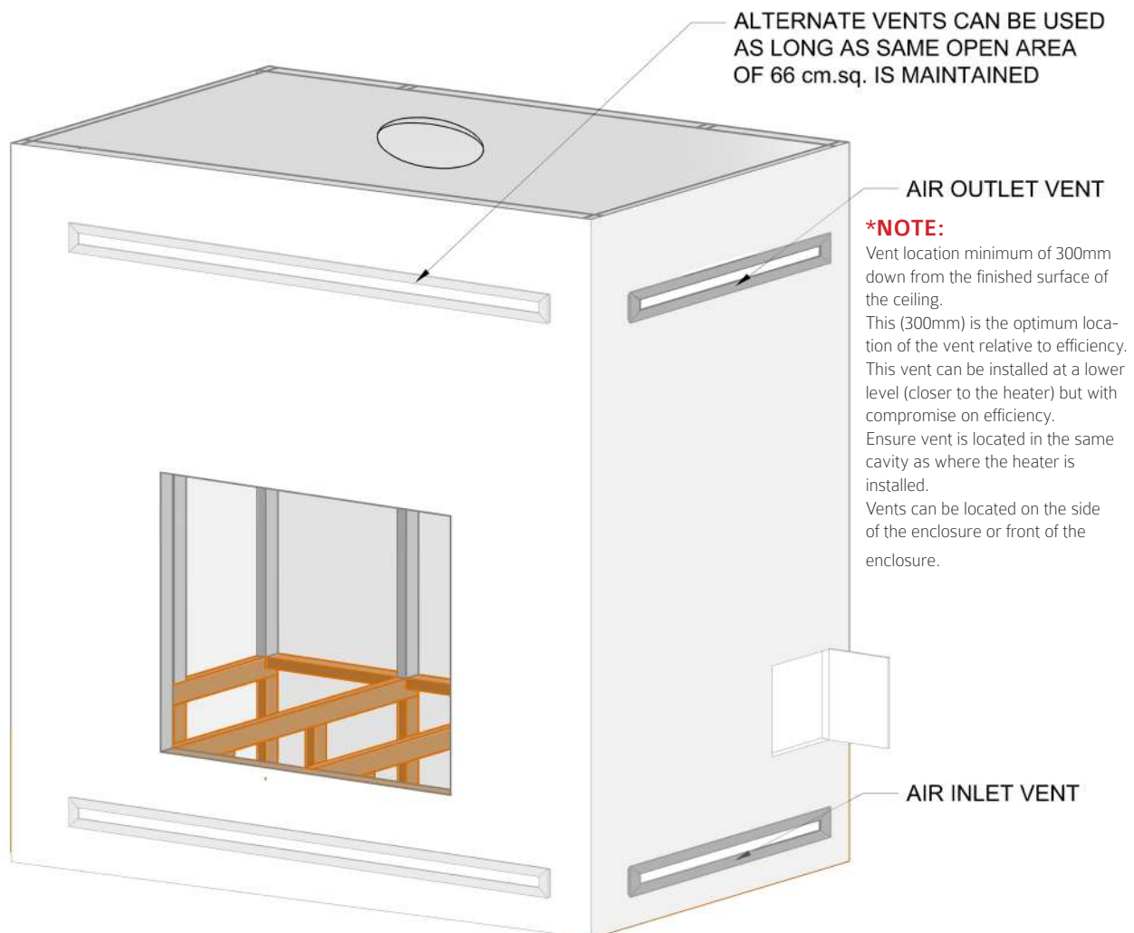
Figure 1.2 (Vents)
